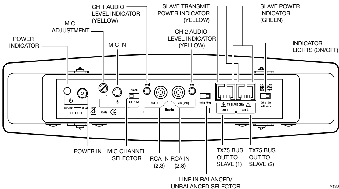
Figure 6: WIR TX75 master rear view
