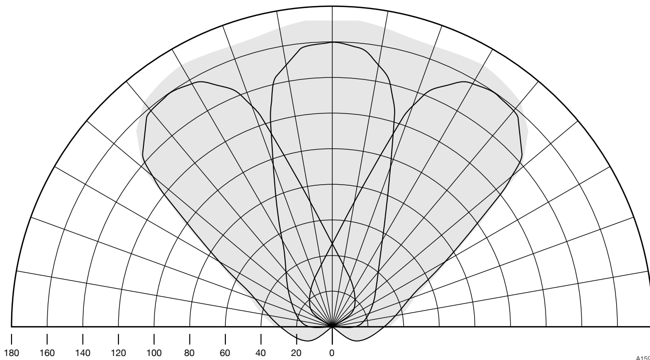
Figure 5: WIR TX75 master and two slaves at an angle of 35° to each other.
