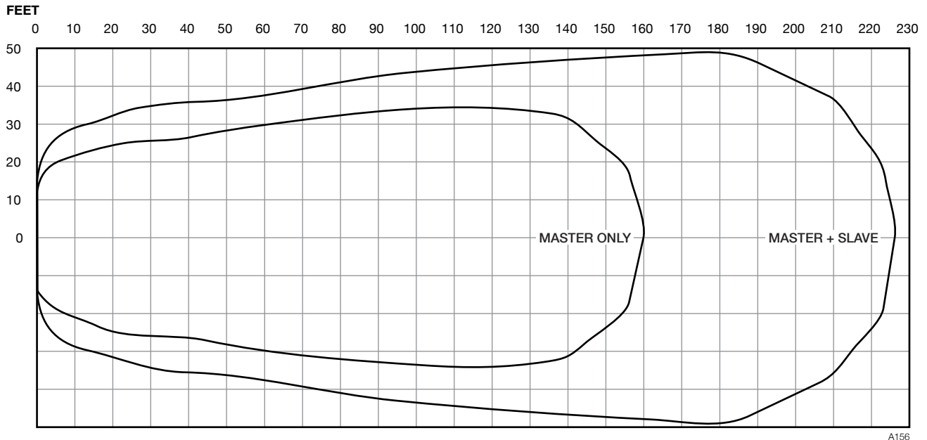
Figure 3: coverage area with second emitter added to same emission point (50% increase)
