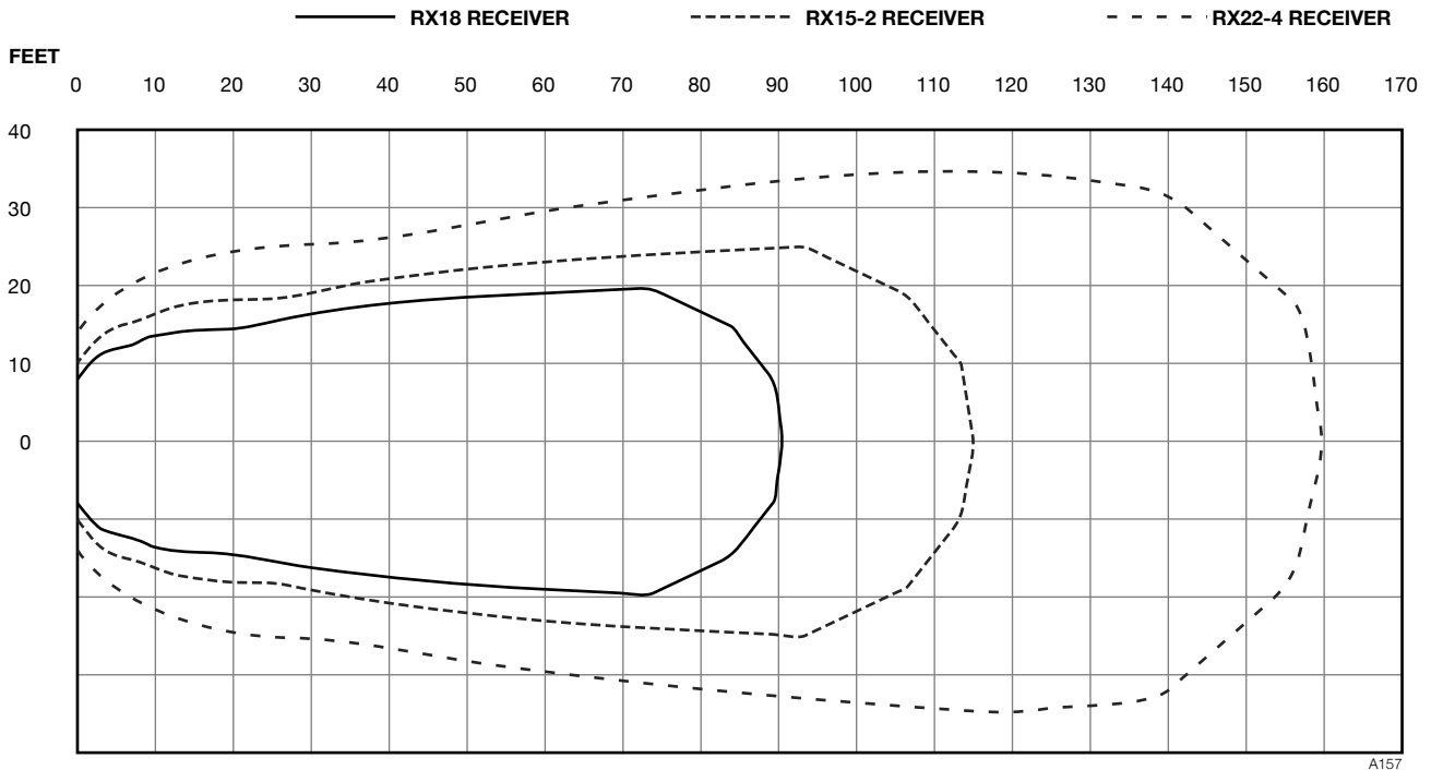
Figure 1: Receiver coverage area with WIR TX75 OR WIR TX75-S transmitter in single channel mode.
