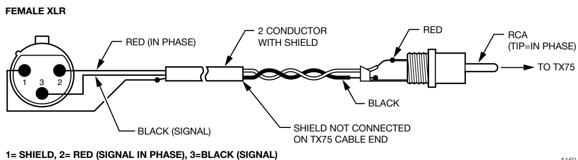
Figure 7: Balanced line out (XLR) to WIR TX75 line input (RCA) cable
