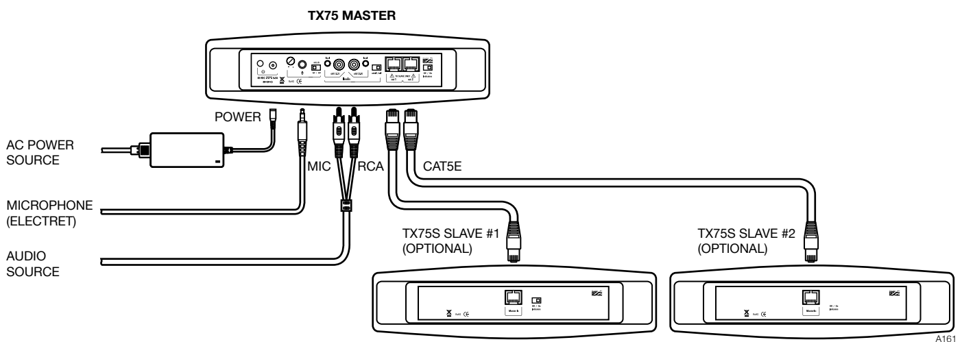
Figure 8: Connecting a WIR TX75 transmitter to two WIR TX75-S slave emitters
